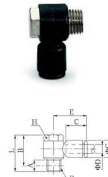
PH 系列 L型回转接头 PH Series Male banjo connector
